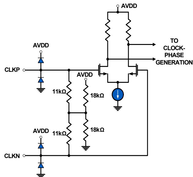
FIGURE 45. CLOCK INPUTS
