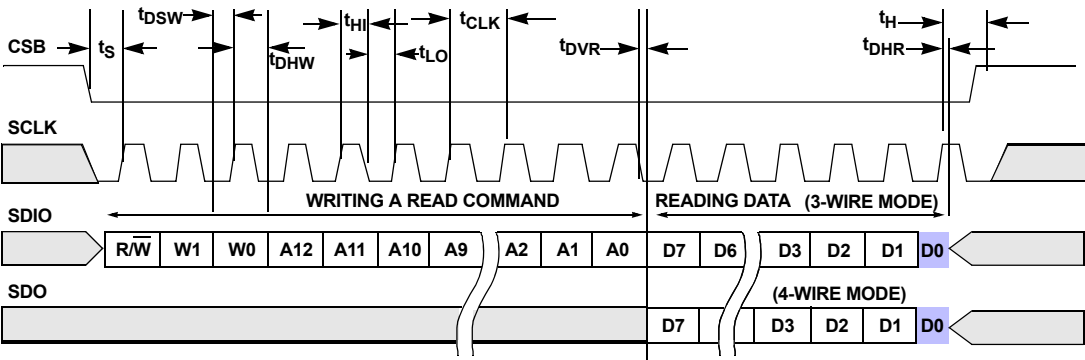
SPI READ
