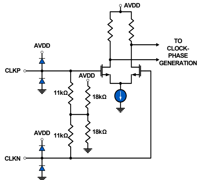
FIGURE 45. CLOCK INPUTS
