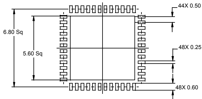
TYPICAL RECOMMENDED LAND PATTERN
