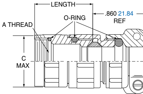
90° ENTRY ROTATABLE COUPLING 2M390MA077
