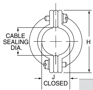
SADDLE CLAMP
