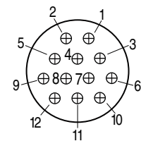
14-12, 16-12, 18-12 (12) #16 Contacts
