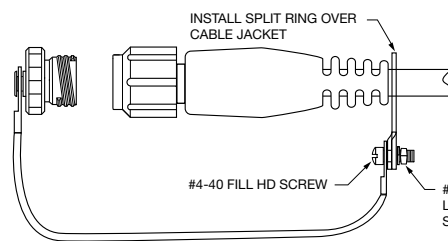
Large Split Ring designed for attaching covers to cables
