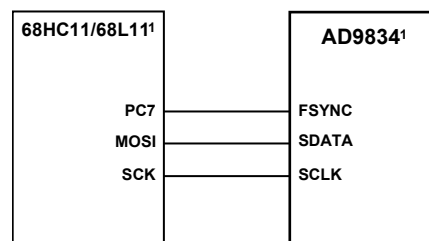
Figure 36. 68HC11/68L11 to AD9834 Interface
