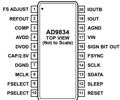
Figure 6. Pin Configuration
