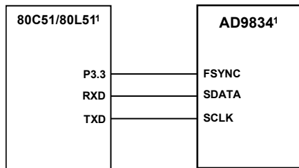
Figure 37. 80C51/80L51 to AD9834 Interface
