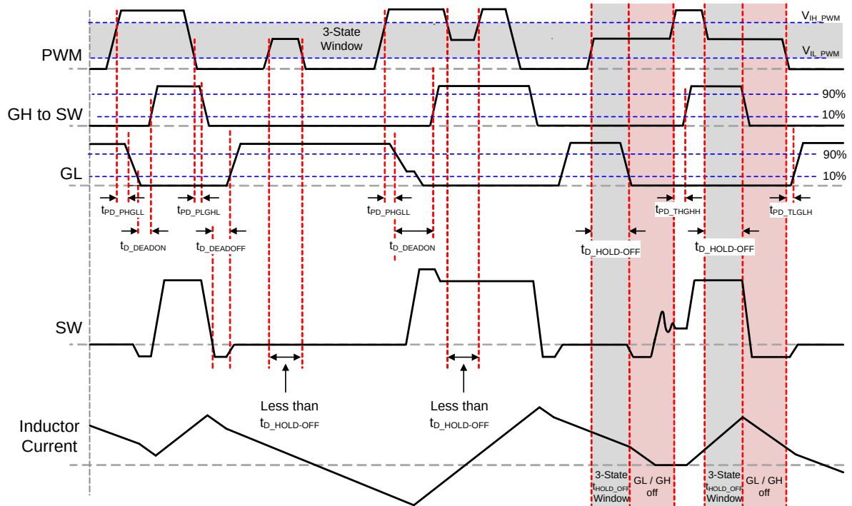
Figure 29. PWM 3-State Timing Diagram (FCCM held HIGH)
