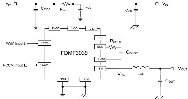
Figure 1. Typical Application Diagram
