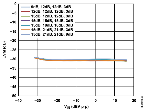
Figure 77. EVM vs. Input Voltage over Digital Gain Settings, Filter Corner = 63 MHz, QPSK, 50 MSPS, 1.5 V p-p Differential Output Level Maintained
