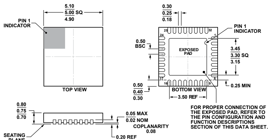
Figure 94. 32-Lead Lead Frame Chip Scale Package [LFCSP_WQ] 5 mm x 5 mm Body, Very Very Thin Quad (CP-32-13) Dimensions shown in millimeters
