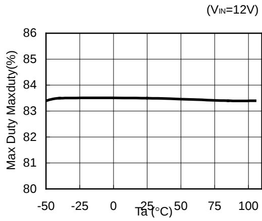
6) Maxduty VS. Temperature R1240x00Xx
