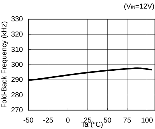
7) Fold-Back Frequency VS. Temperature R1240x00XB
