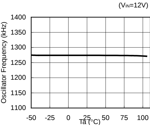
5) Oscillator Frequency VS. Temperature R1240x00Xx
