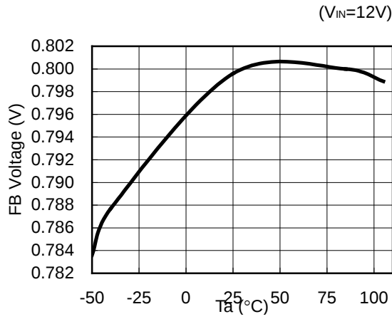
4) FB Voltage VS. Temperature R1240x00Xx
