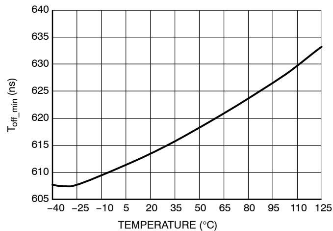
Figure 32. Minimum Off Time @ R_{t\_off\_min} = 0\text{ }\Omega
