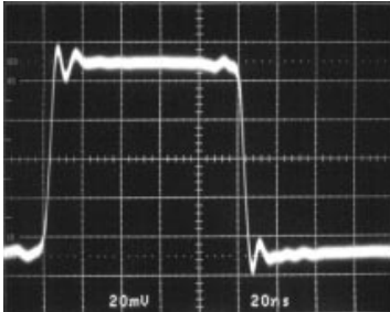
R_G = 0 V_{IN} = 100\text{mV} V_S = \pm 15\text{V} f = 5\text{MHz} LT1220 • TPC19
