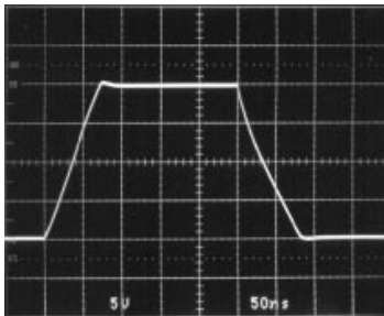
R_F = R_G = 1\text{k} V_{IN} = 20\text{V} V_S = \pm 15\text{V} f = 2\text{MHz} LT1220 • TPC23
