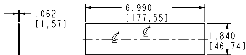
REAR PANEL
