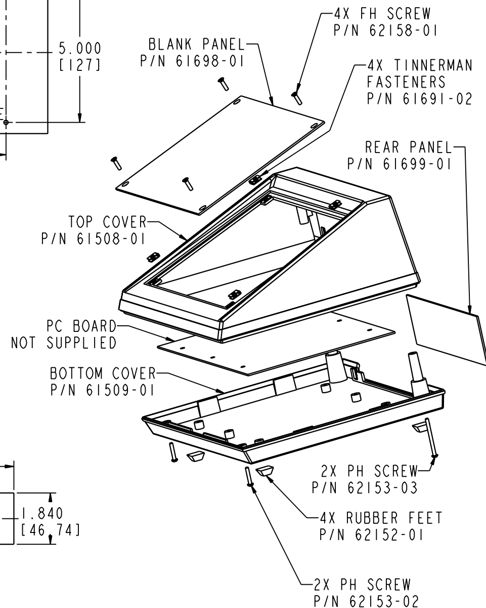
REAR PANEL
