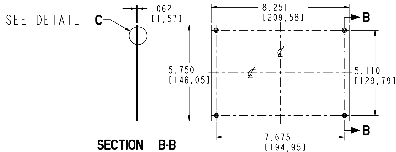
BLANK PANEL
