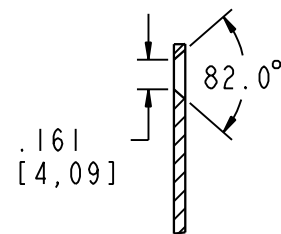
DETAIL C SCALE 2.000 4 PLACES
