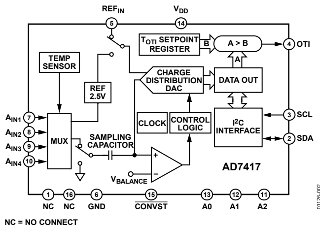
Figure 2. AD7417
