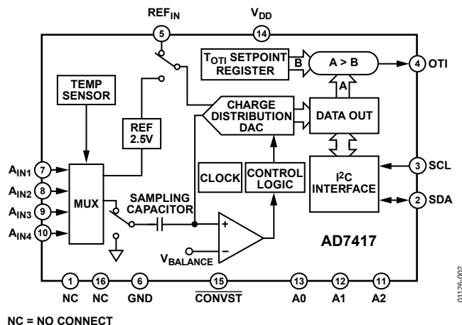
Figure 2. AD7417
