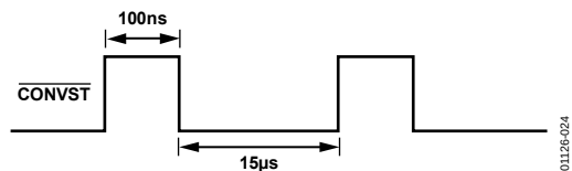
Figure 22. \overline{\text{CONVST}} When VIN Channel Selected
