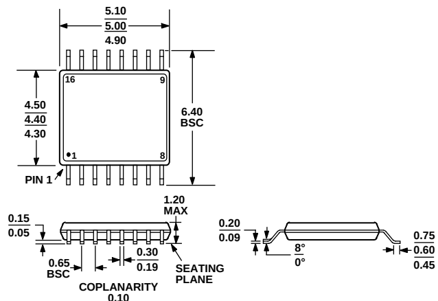
Figure 28. 16-Lead Thin Shrink Small Outline Package [TSSOP] (RU-16)
