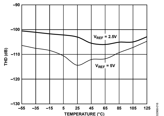
Figure 18. THD vs. Temperature
