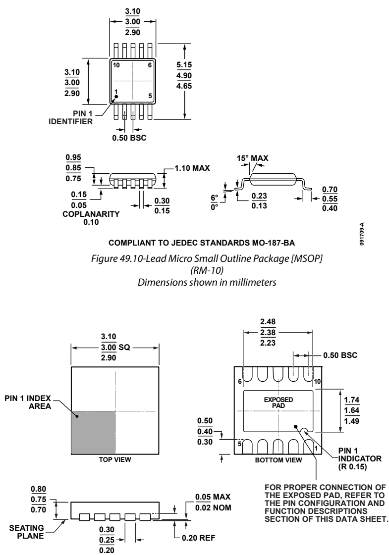
Figure 50. 10-Lead Lead Frame Chip Scale Package [QFN (LFCSP_WD)] 3 mm × 3 mm Body, Very Very Thin, Dual Lead (CP-10-9)
