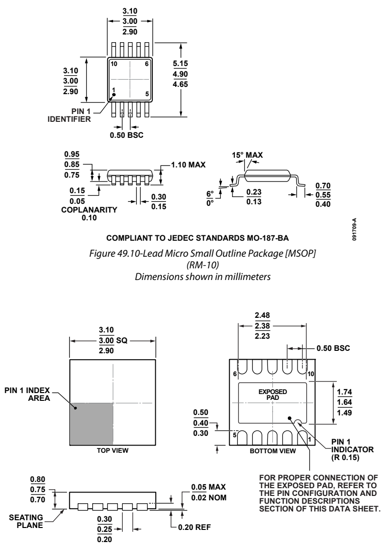
Figure 50. 10-Lead Lead Frame Chip Scale Package [QFN (LFCSP_WD)] 3 mm × 3 mm Body, Very Very Thin, Dual Lead (CP-10-9) Dimensions shown in millimeters
