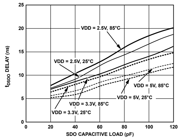
Figure 24. t_{\text{SDO}} Delay vs. Capacitance Load and Supply
