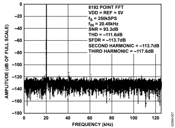
Figure 9. FFT Plot
