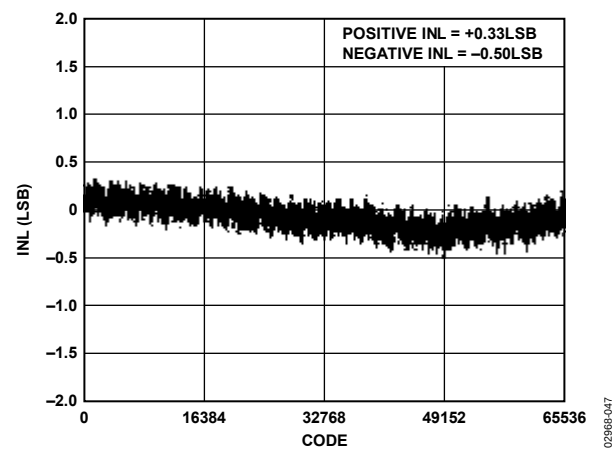
Figure 7. Integral Nonlinearity vs. Code
