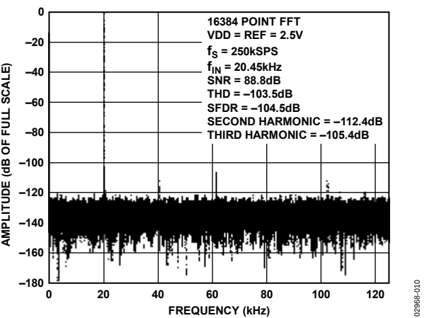
Figure 12. FFT Plot
