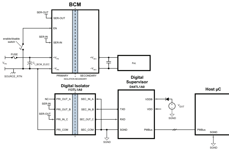
BCM6123xD1E13A3y01 at point-of-load
