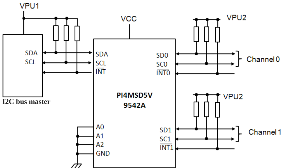
Figure 3. Typical Application
