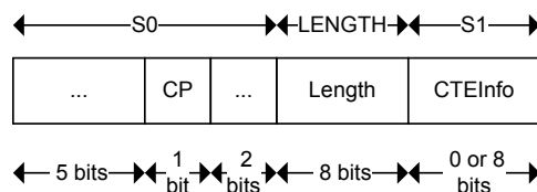
Figure 72: Data channel PDU header
