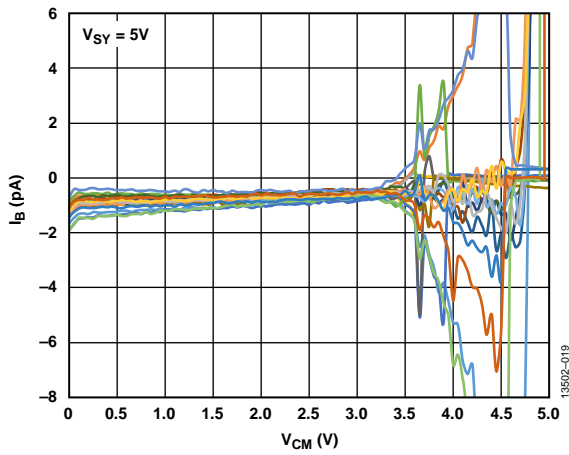
Figure 18. Input Bias Current ( I_b ) vs. Input Common-Mode Voltage ( V_{CM} ), V_{SY} = 5 V
