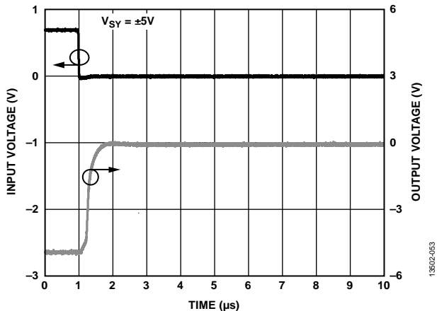
Figure 52. Negative Overload Recovery, A_V = -10 , V_{SV} = \pm 5 V
