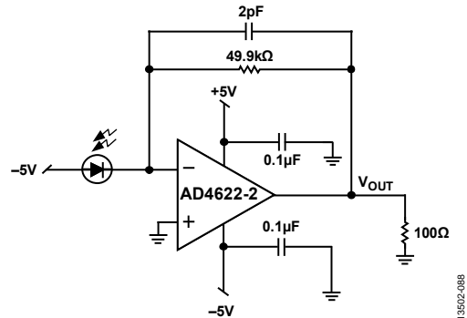
Figure 87. Photodiode Preamplifier
