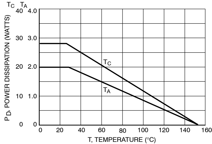
Figure 1. Power Derating
