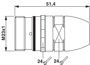
Dimensional drawing
