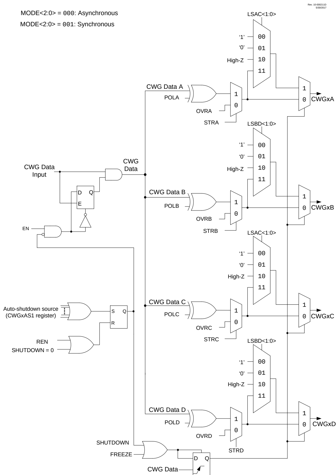
Figure 31-9. Simplified CWG Block Diagram (Output Steering Modes)
