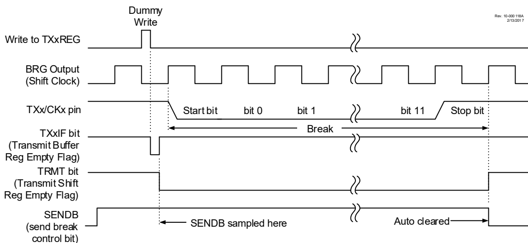
Figure 36-9. Send Break Character Sequence
