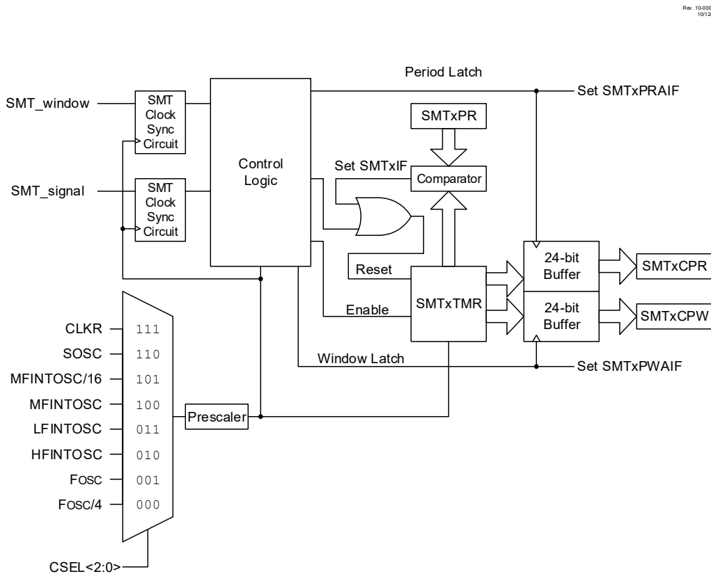
Figure 37-1. Signal Measurement Timer Block Diagram
