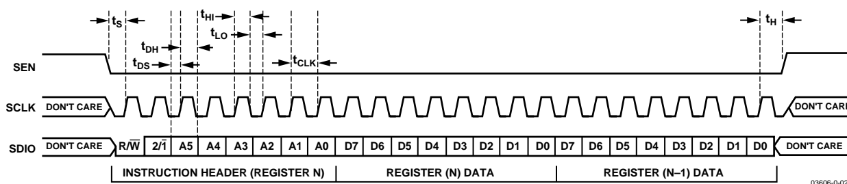
Figure 79. 2-Byte Serial Register Write in MSB First Mode
