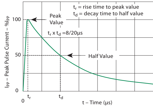
Figure 6 - Pulse Waveform
