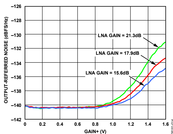
Figure 14. Short-Circuit, Output-Referred Noise vs. GAIN+
