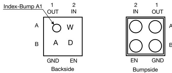
Figure 2 - WCSP 2 x 2 Package
