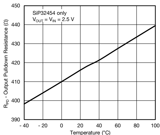
Output Pulldown Resistance vs. Temperature
