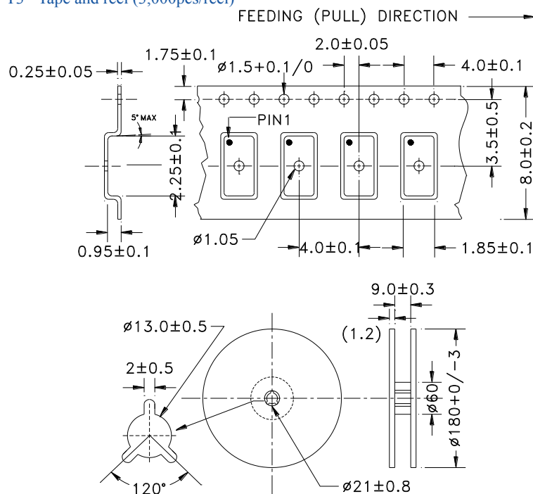
Dimensions: mm
