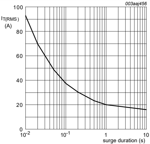
Fig. 3. RMS on-state current as a function of surge duration; maximum values f = 50 \text{ Hz}; T_h = 86 \text{ °C}
