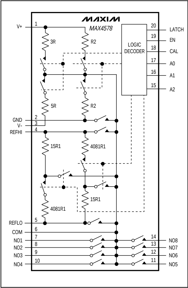
Pin Configurations/ Functional Diagrams (continued)
