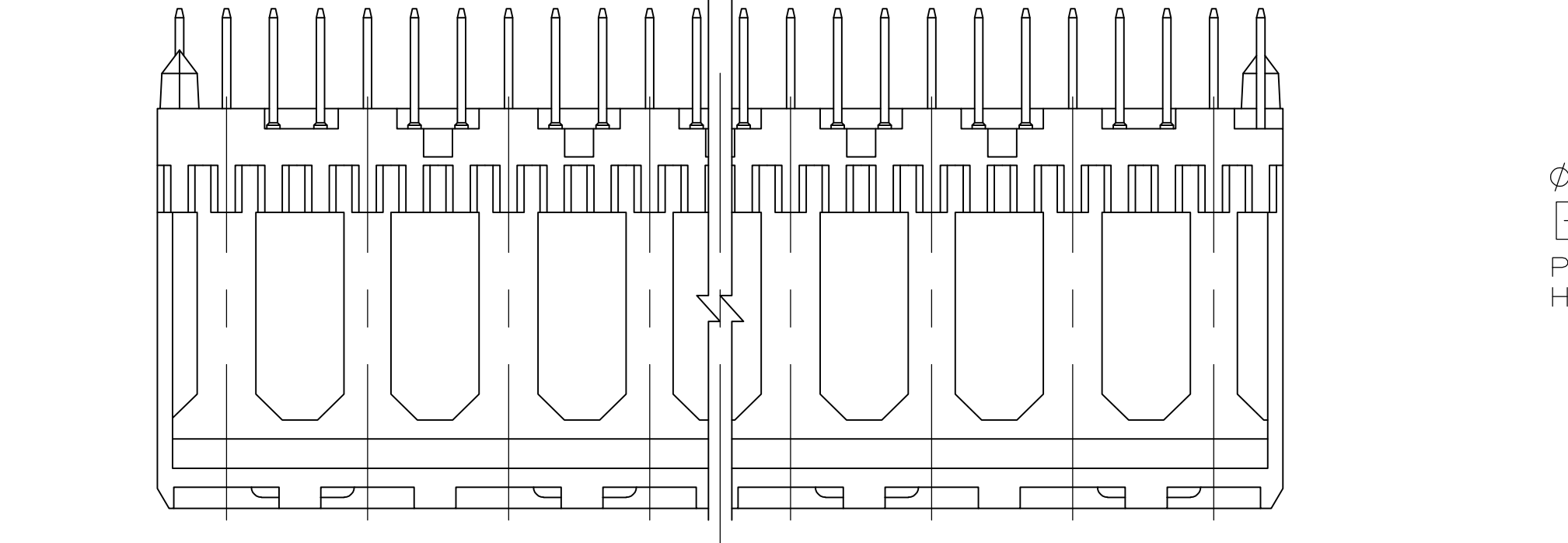
RECOMMENDED CIRCUIT PATTERN (COMPONENT SIDE)
