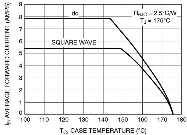
Figure 7. Current Derating
