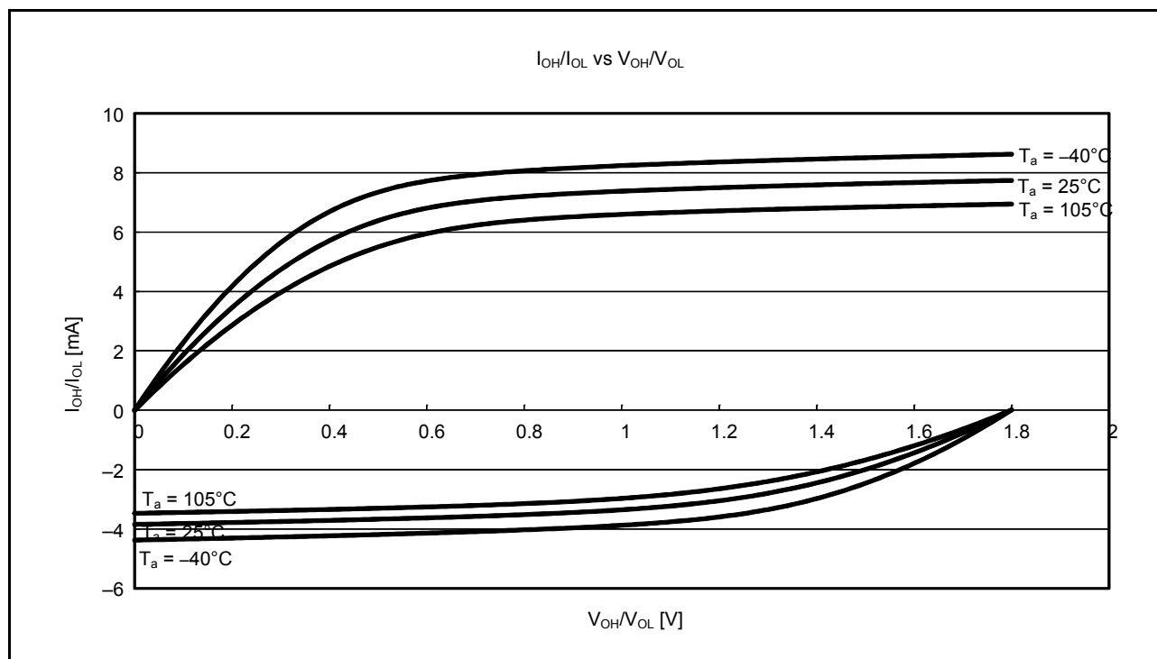
Figure 5.13 V_{OH}/V_{OL} and I_{OH}/I_{OL} Temperature Characteristics of General Ports (Except for the RIIC Output Pin, Ports P40 to P44, P46, Ports PJ6, PJ7) at V_{CC} = 1.8 V (Reference Data)
