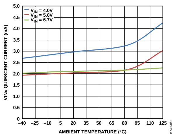
Figure 15. V_{INx} Quiescent Current vs. Ambient Temperature, LDO Mode
