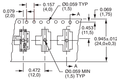
CARRIER TAPE
