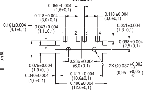
JSM08022SAQNL SPDT Surface Mount Momentary only
