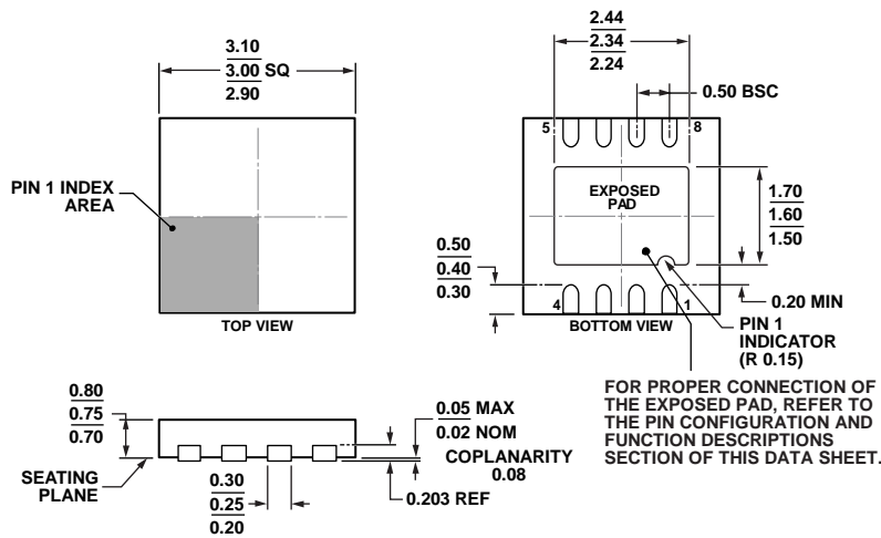
Figure 92. 8-Lead Lead Frame Chip Scale Package [LFCSP_WD] 3 mm x 3 mm Body, Very Very Thin, Dual Lead (CP-8-11)
