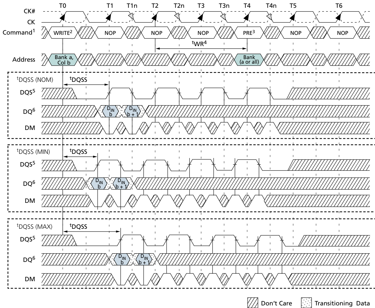
Figure 44: WRITE-to-PRECHARGE – Interrupting
