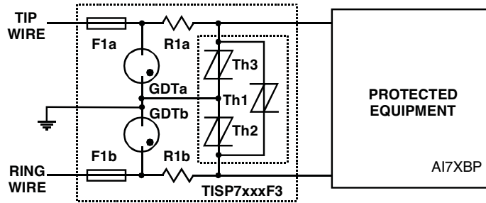
Figure 36. Protection Module
