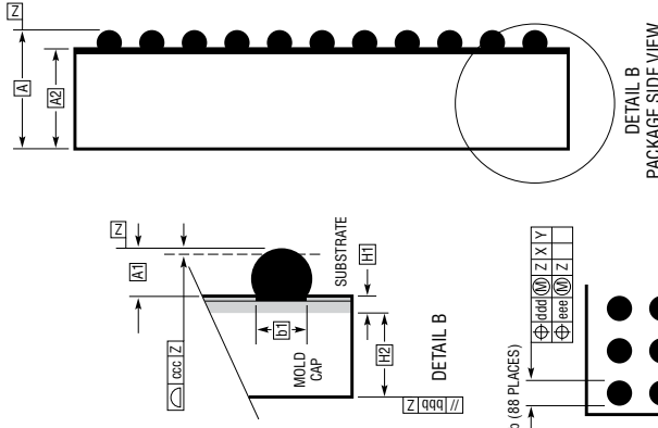
BGA Package 88-Lead (15mm × 11.25mm × 5.01mm) (Reference LTC DWG # 05-08-1541 Rev A)
